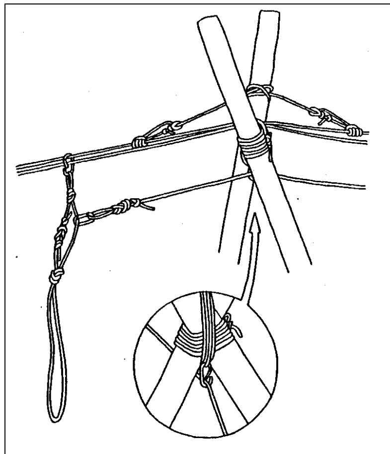
Carrying Rope with Belay Rope Attached
