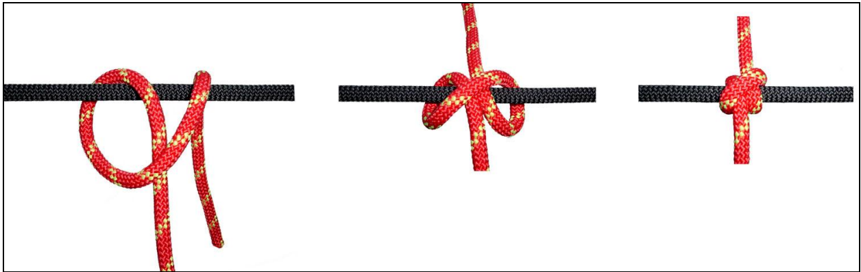
End of rope clove hitch
