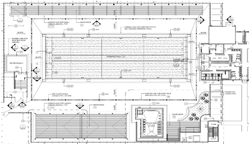
Floor Plan
