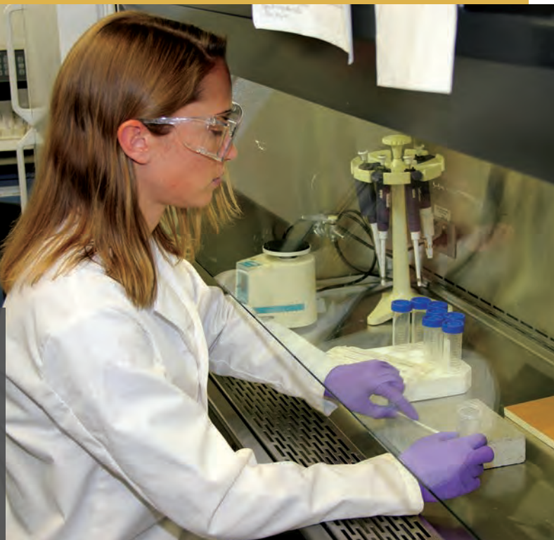
Enclosed biosafety cabinets ventilate any potentially pathogens away from the operator and into carbon filters.
