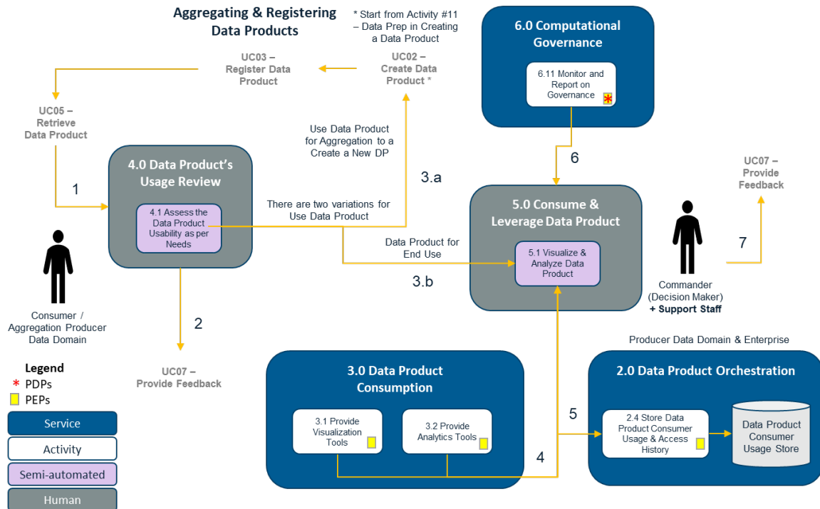
Figure 14. Use Case Activity Diagram: UC06 – Consume Data Product
