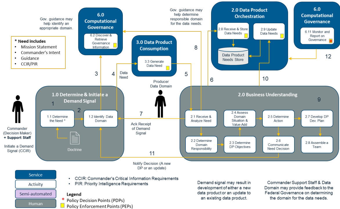
Figure 9. Use Case Activity Diagram: UC01 – Identify Data Product Need
