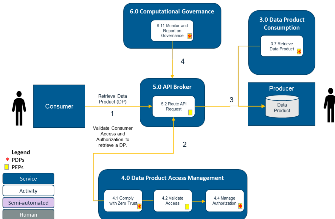
Figure 13. Use Case Activity Diagram: UC05 – Retrieve Data Product
