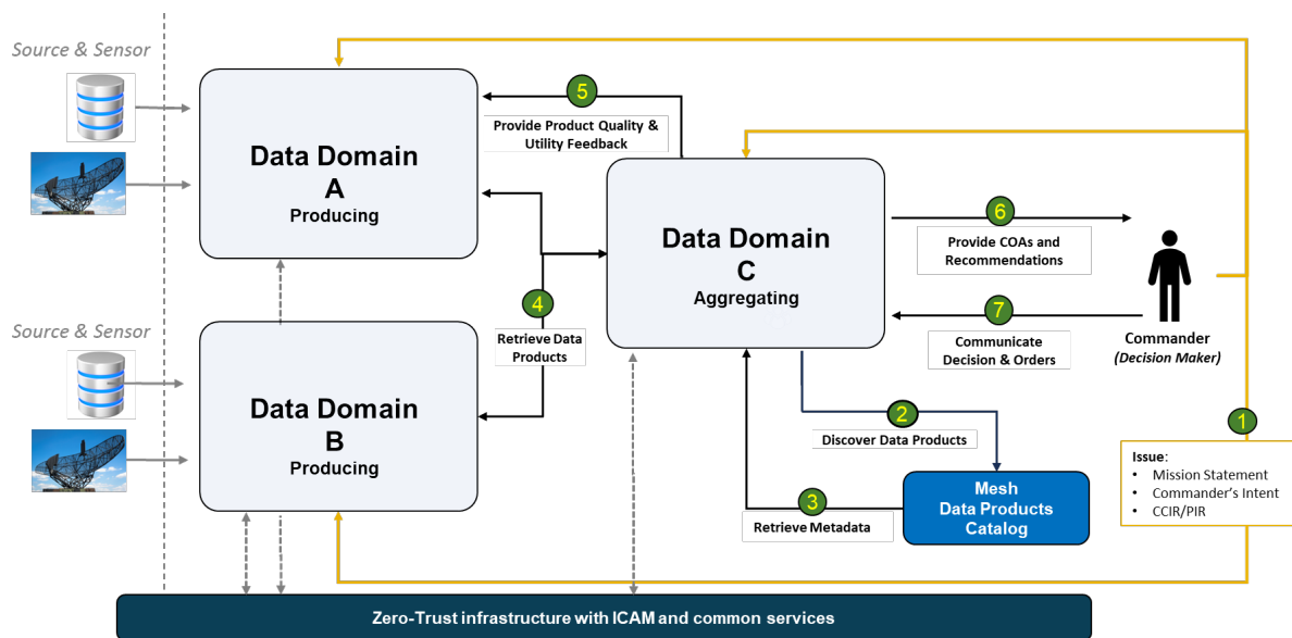
Figure 4. Data Product Orchestration
