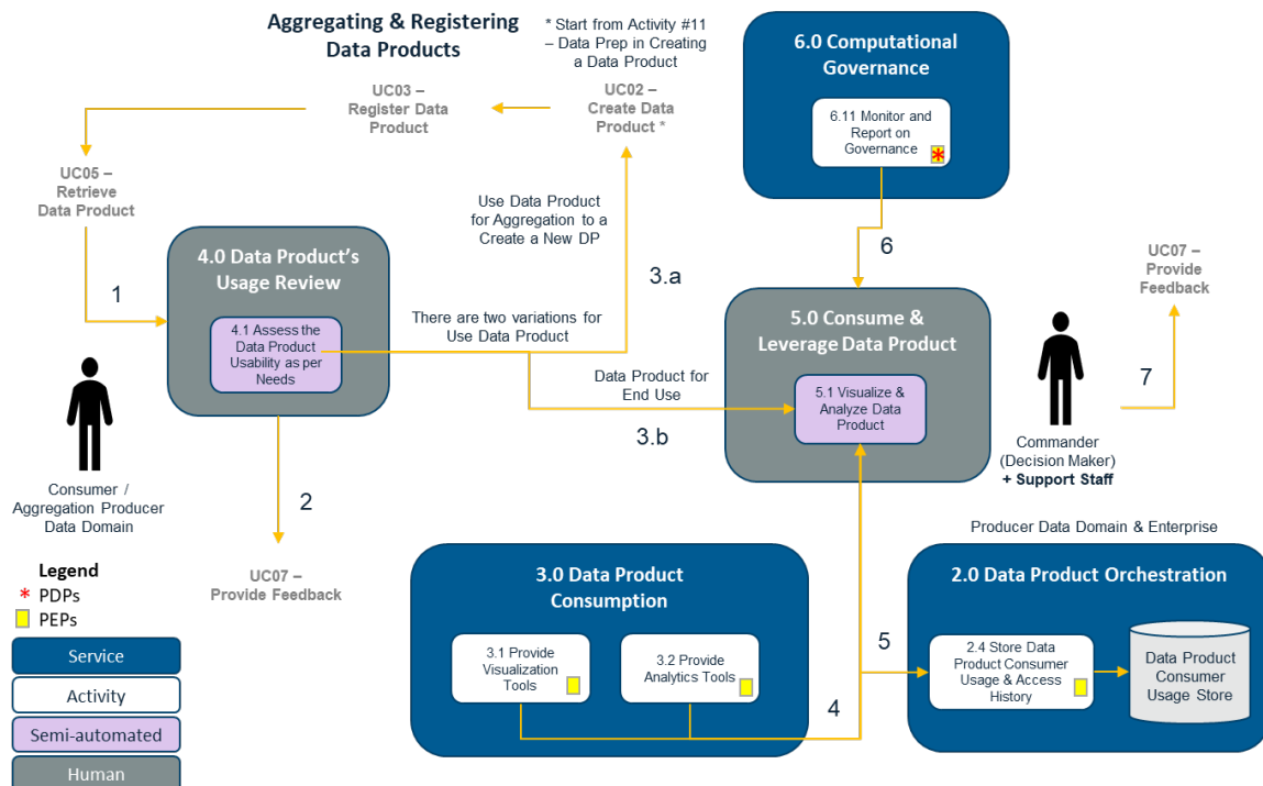
Figure 14. Use Case Activity Diagram: UC06 – Consume Data Product
