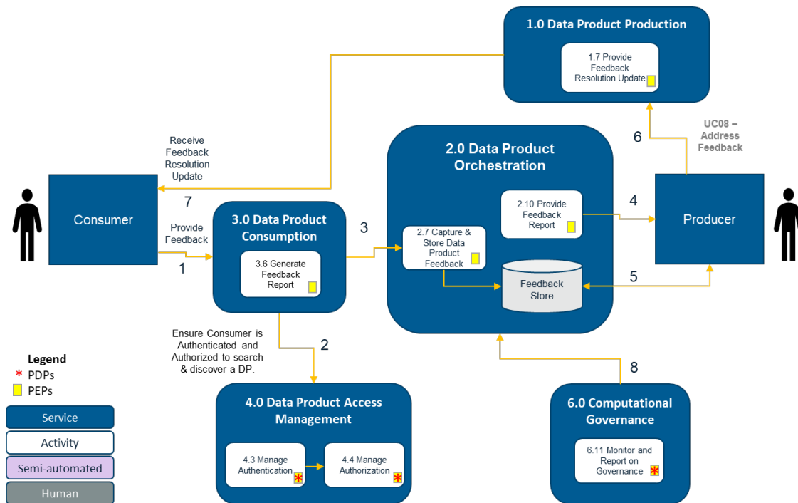
Figure 15. Use Case Activity Diagram: UC07 – Provide Feedback
