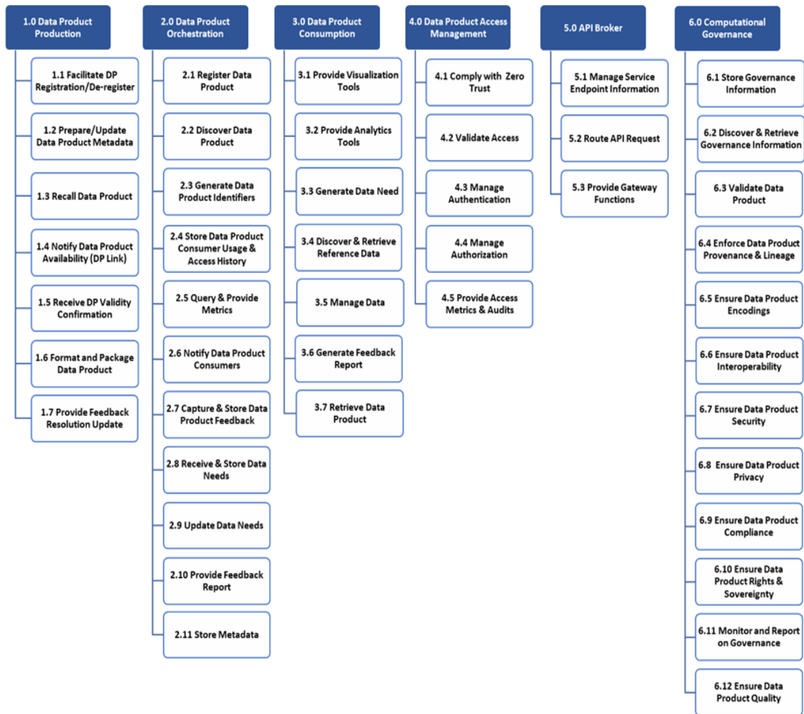
Figure 5. Service Activity Decomposition
