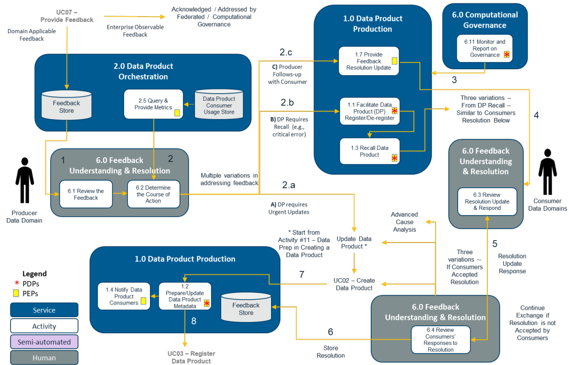
Figure 16. Use Case Activity Diagram: UC08 – Address Feedback
