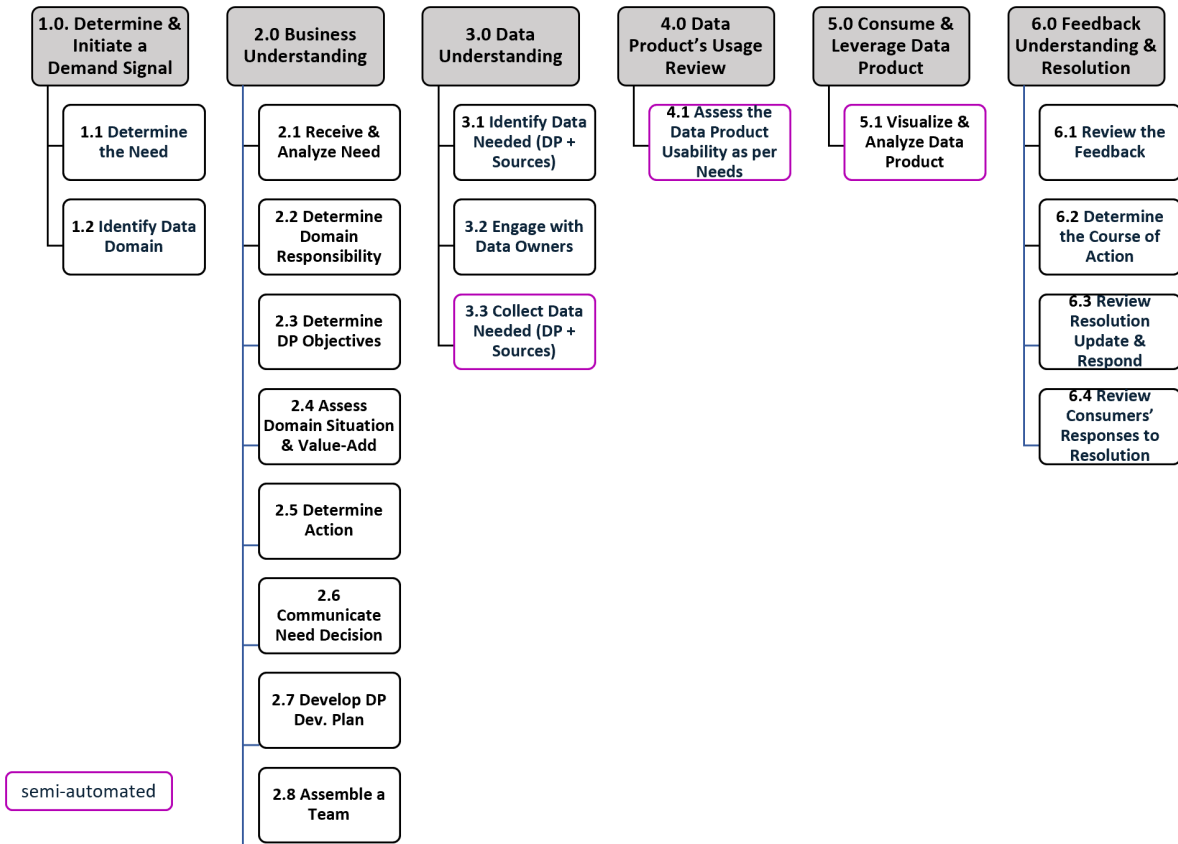
Figure 6. Decomposition of Domain Processes
