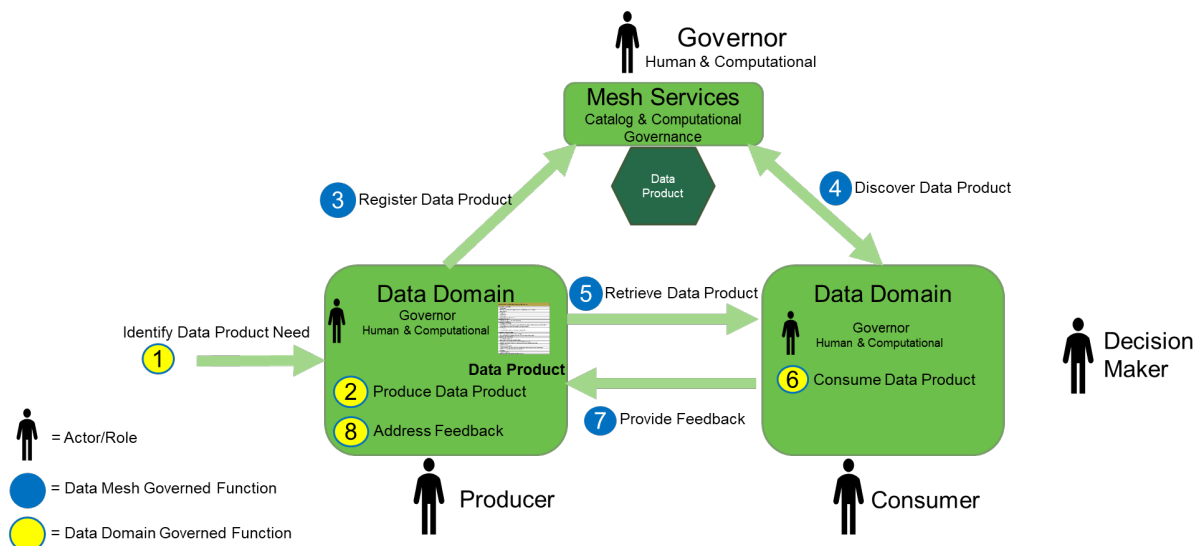
Figure 2. Data Mesh Key Functions, Actors, and Roles
