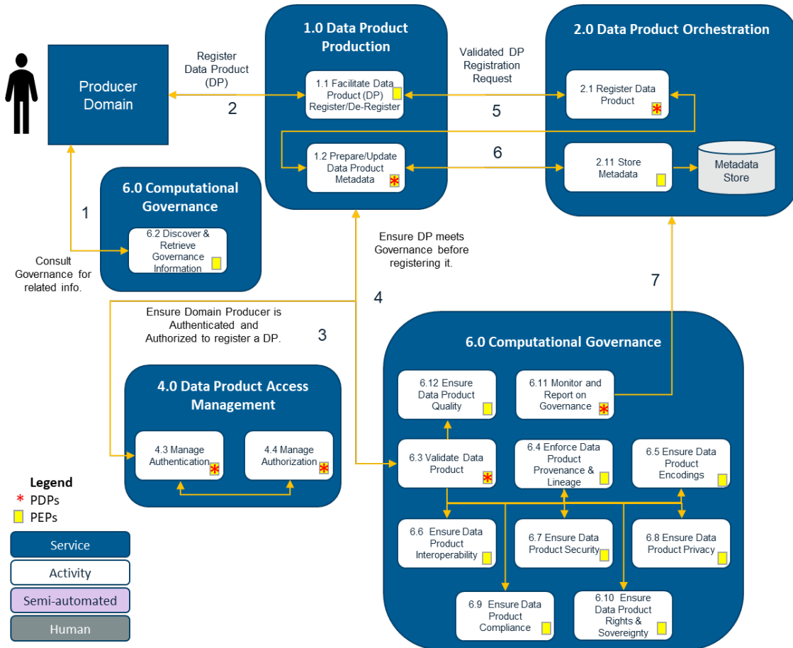
Figure 11. Use Case Activity Diagram: UC03 – Register Data Product
