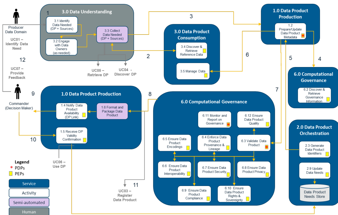
Figure 10. Use Case Activity Diagram: UC02 – Produce Data Product
