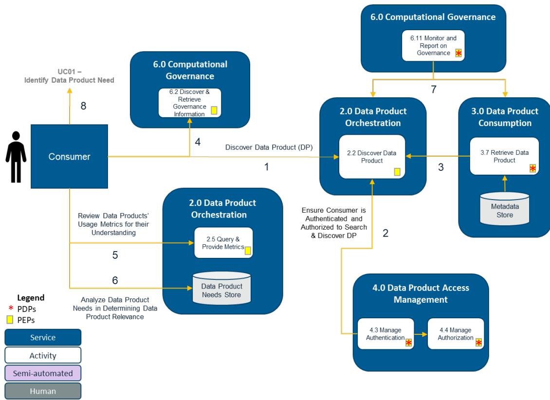
Figure 12. Use Case Activity Diagram: UC04 – Discover Data Product
