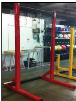
Figure D-9. One per lane. Squat stand 92 inches in height offers ample space for pull-ups under an 8-foot ceiling with a compact 8 inch x 48 inch base footprint that can be easily transported or relocated.
